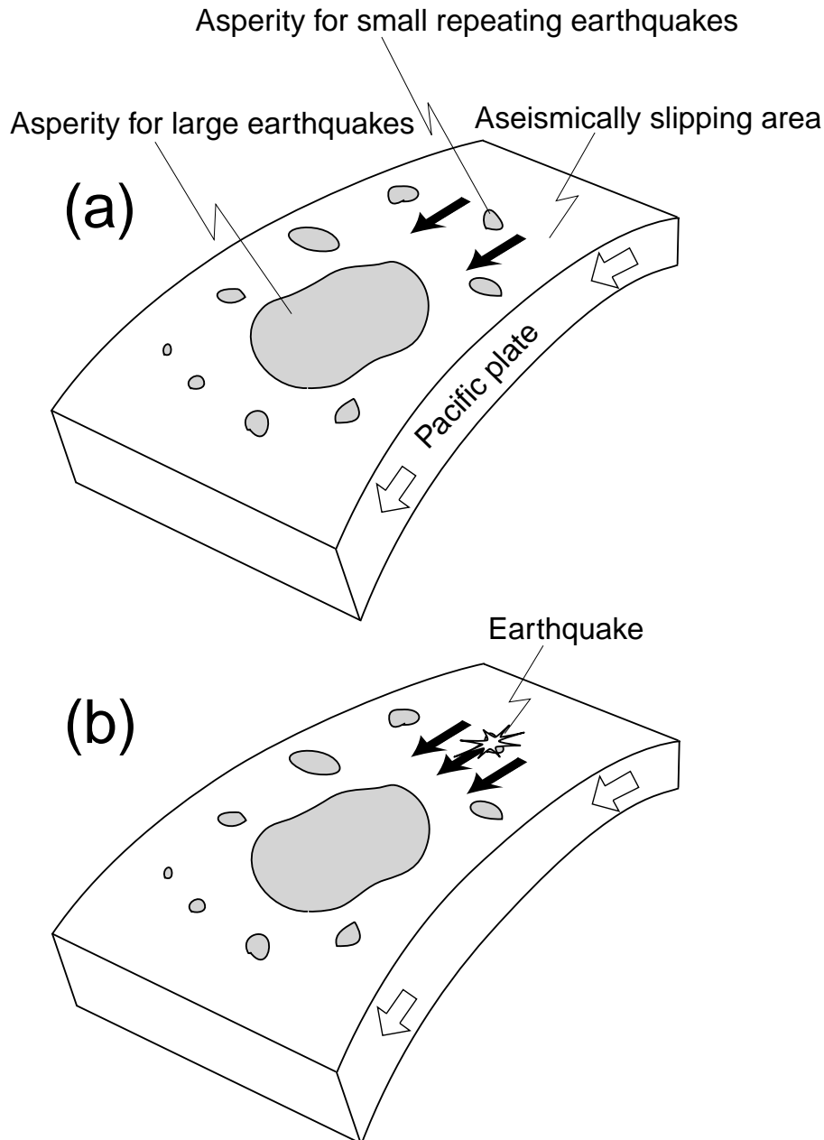
Fig. 1. Schematic illustration showing the relation between slips in the aseismic area and asperities on the plate boundary east off northern Honshu, Japan. Various sizes of asperities are distributed on the plate boundary. (a) Areas other than asperities slip aseismically, and (b) the asperities eventually rupture as earthquakes.
