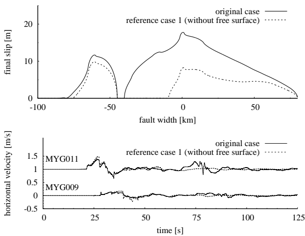
Fig. 10. Comparison of simulation results between original case and reference case 1 (without free surface); final slip distribution (top) and synthetic velocity waveforms (bottom).
