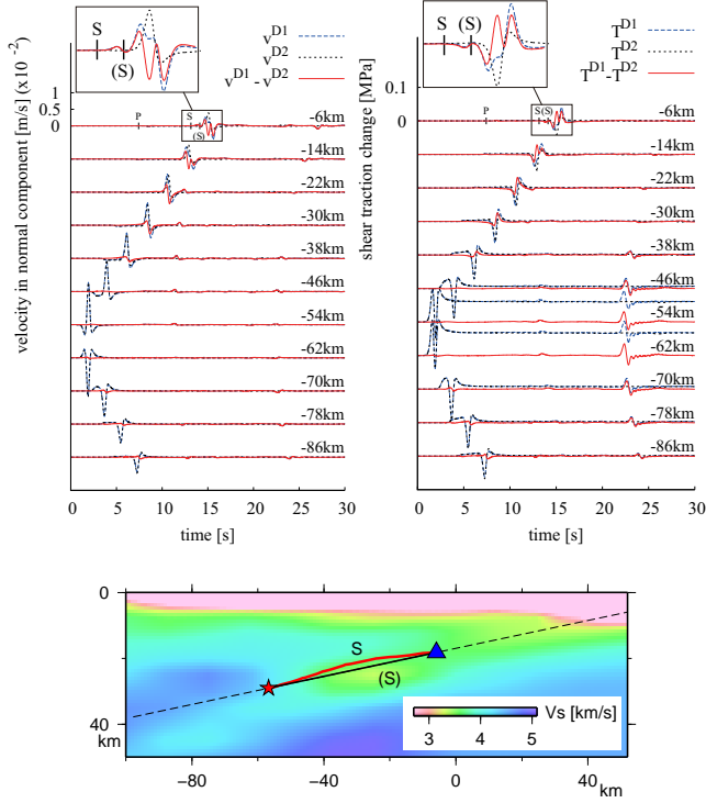
Fig. 4. Characteristics of perturbation terms calculated from the differences between solutions from the target model (D1) and the layered model (D2); velocities in normal component and shear traction changes observed along the fault plane (top). A double-couple point source is located at -58 km along the fault width. Seismic ray traces of S-wave for D1, S, and for D2, (S) (bottom).
