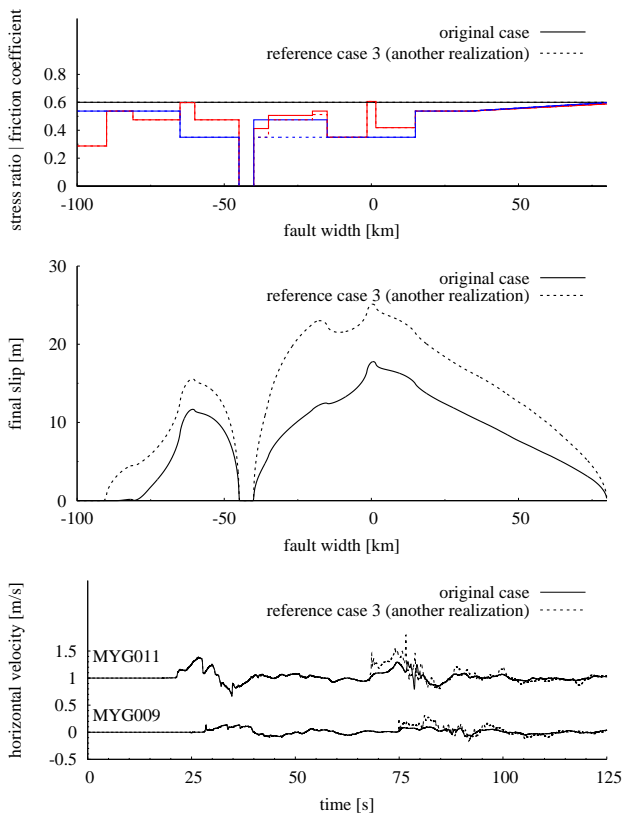
Fig. 12. Comparison of simulation results between original case and reference case 3 (another realization); friction coefficient (top), final slip distribution (middle) and synthetic velocity waveforms (bottom).
