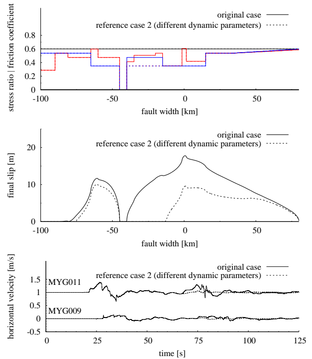
Fig. 11. Comparison of simulation results between original case and reference case 2 (different dynamic parameters); friction coefficient (top), final slip distribution (middle) and synthetic velocity waveforms (bottom).
