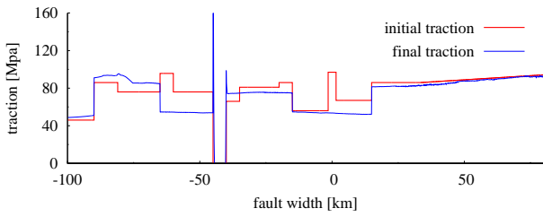
Fig. 7. Comparison of initial and final shear tractions. The differences indicate the stress drop of the simulation.
