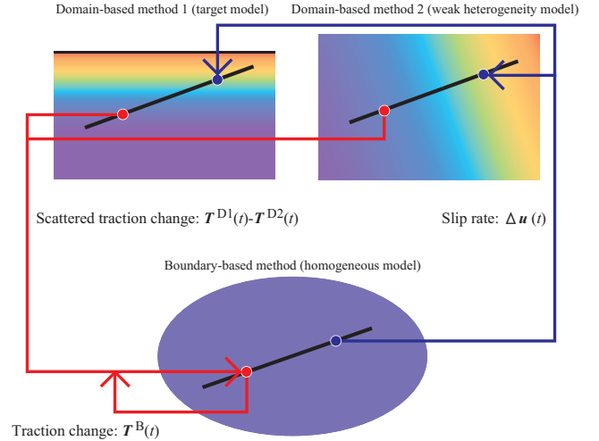
Fig. 1. Calculation procedure of pseudo-BDM (pBDM). pBDM requires parallel three calculations: 1) a boundary-based method for a homogeneous full space (bottom), 2) a domain-based method for the target model (left top), and 3) a domain-based method for a weak heterogeneity model represented by a layered structure (right top). Color gradations in top figures are conceptual map of material heterogeneity, such as velocity structures as shown in Fig.2. An instantaneous traction change is represented by combination of a direct term calculated from the boundary-based method and a residual term calculated from the differences between two solutions of the domain-based methods.
