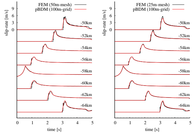
Fig. 5. Comparison of slip-rate time histories calculated by pBDM and FEM. The mesh size of FEM is set to be 50 m (left), and 25 m (right).
